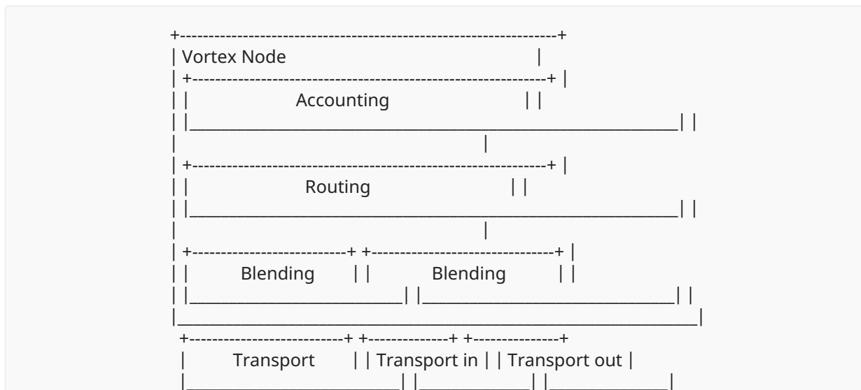
Figure 1: Layer overview
